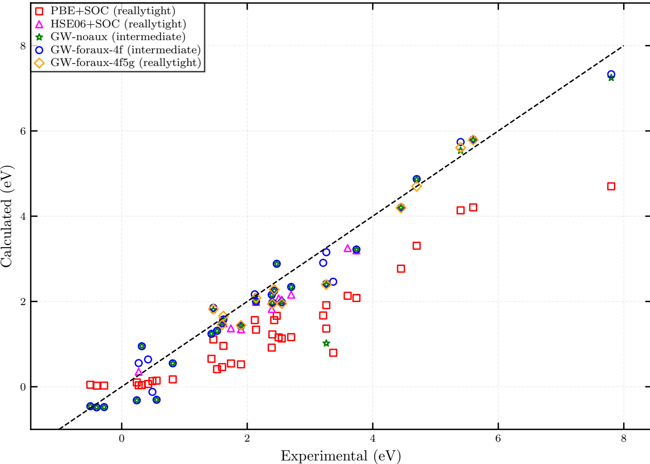
GW band gaps of compound semiconductors
